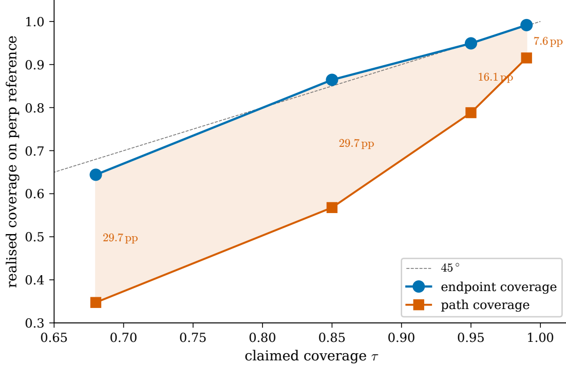
Figure 8: Path coverage gap on the 24/7 stock-perp reference. Endpoint coverage (blue) tracks nominal across \tau \in \{0.68, 0.85, 0.95, 0.99\} on the perp-listed subset; path coverage (vermillion) — the fraction of weekends where the perp 1m bar high/low stay inside the served band over the full [Fri 16:00, Mon 09:30] window — runs 29.7/29.7/16.1/7.6 pp behind. The gap collapses meaningfully only at \tau = 0.99 . Sample is small ( n = 118 symbol-weekends across 19 calendar weekends, 2025-12 to 2026-04); the read is directional and §10.2 (the path-fitted conformity score) is the methodology fix.
